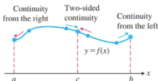
FIGURE 2.56 Continuity at points a , b , and c .
