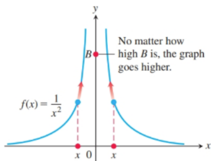
FIGURE 2.46 The graph of f(x) in Example 11 approaches infinity as x \rightarrow 0 .
