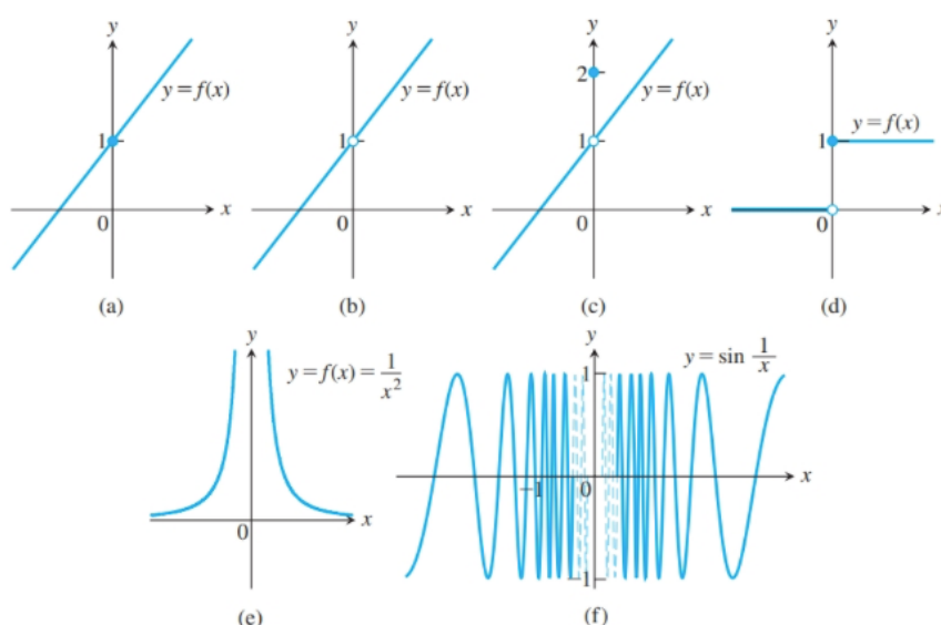
FIGURE 2.60 The function in (a) is continuous at x = 0 ; the functions in (b) through (f) are not.
