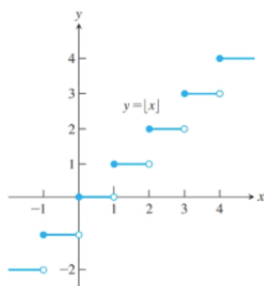
FIGURE 2.59 The greatest integer function is continuous at every noninteger point. It is right-continuous, but not left-continuous, at every integer point (Example 4).
