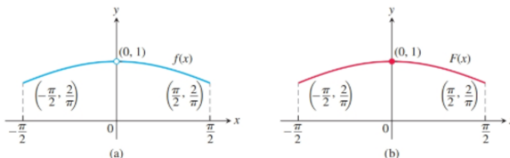
FIGURE 2.67 (a) The graph of f(x) = (\sin x)/x for -\pi/2 \leq x \leq \pi/2 does not include the point (0, 1) because the function is not defined at x = 0 . (b) We can extend the domain to include x = 0 by defining the new function F(x) with F(0) = 1 and F(x) = f(x) everywhere else. Note that F(0) = \lim_{x \rightarrow 0} f(x) and F(x) is a continuous function at x = 0 .
