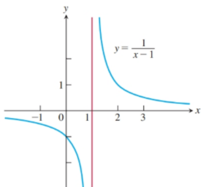
FIGURE 2.45 Near x = 1 , the function y = 1/(x - 1) behaves the way the function y = 1/x behaves near x = 0 . Its graph is the graph of y = 1/x shifted 1 unit to the right (Example 10).
