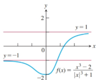
FIGURE 2.39 The graph of the function in Example 4 has two horizontal asymptotes.
