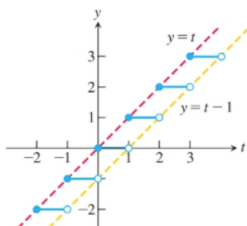
FIGURE 2.41 The graph of the greatest integer function y = [t] is sandwiched between y = t - 1 and y = t .
