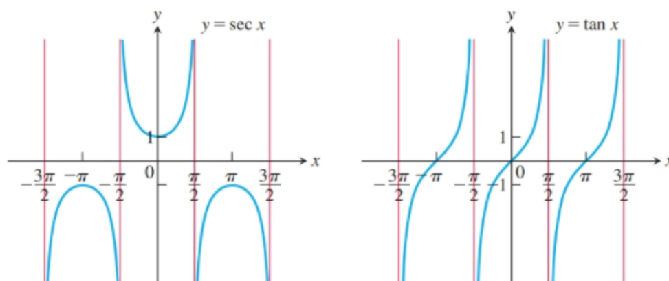
FIGURE 2.52 The graphs of \sec x and \tan x have infinitely many vertical asymptotes (Example 17).
