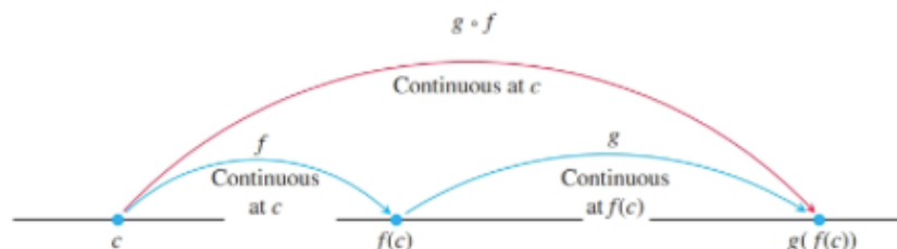
FIGURE 2.62 Compositions of continuous functions are continuous.
