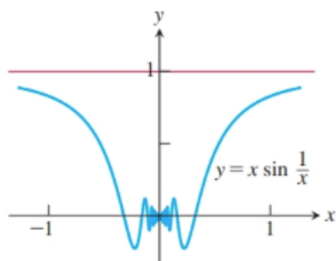
FIGURE 2.40 The line y = 1 is a horizontal asymptote of the function graphed here (Example 5b).
