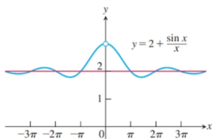
FIGURE 2.42 A curve may cross one of its asymptotes infinitely often (Example 7).
